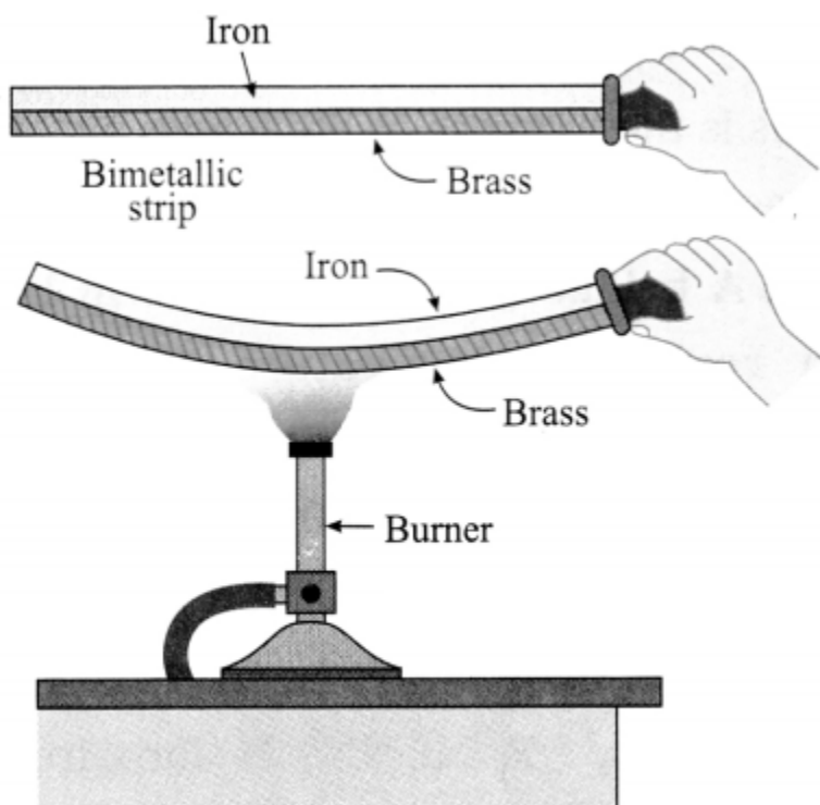
A bimetallic strip
