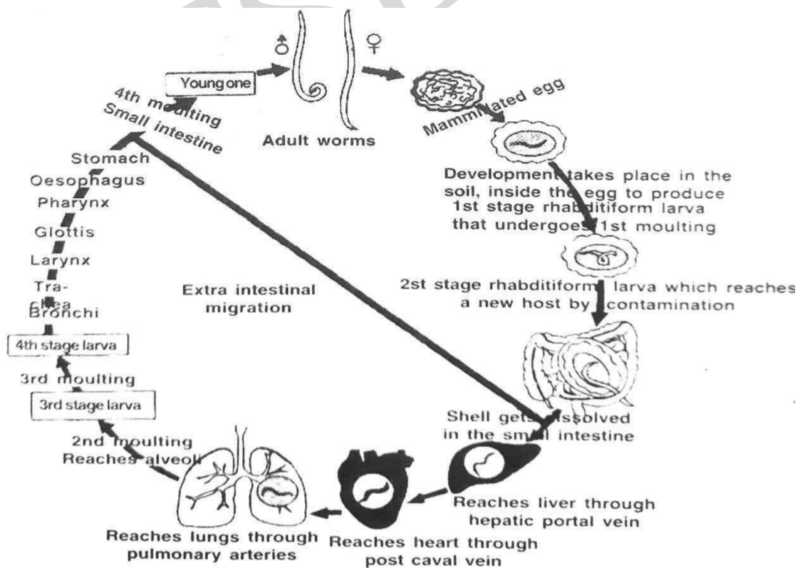
Life cycle of Ascaris lumbricoides
