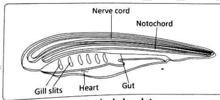
Typical chordate
