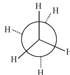
Newman Projection
