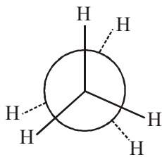
Newman Projection
