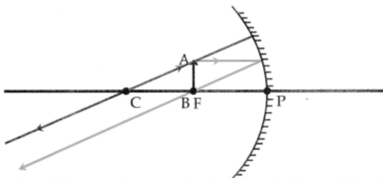
Object at focus for a concave mirror.
