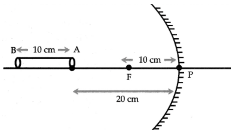
Object in front of a concave mirror
