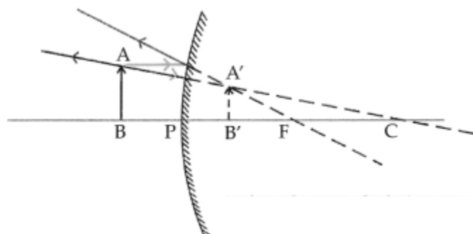
Object between Infinity and P of a Convex mirror
