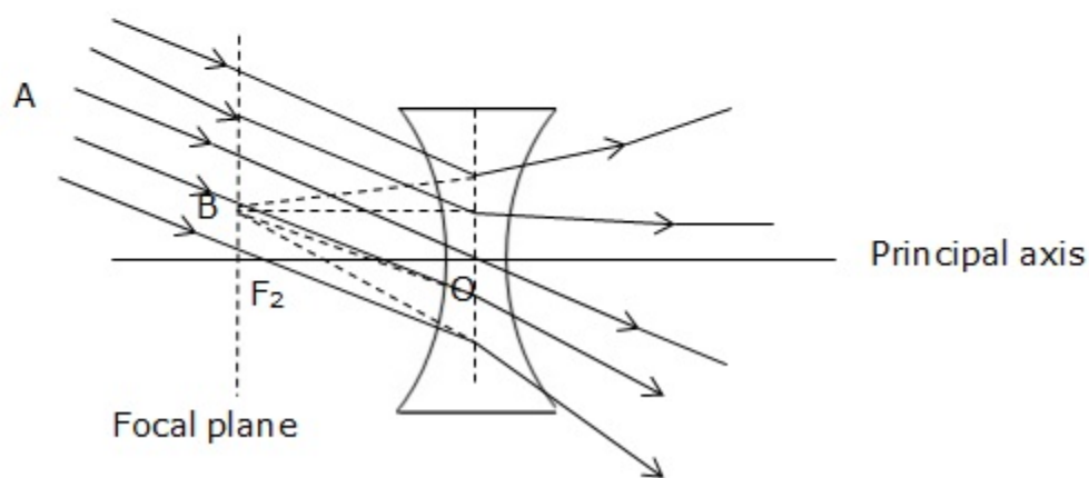
Refraction of an oblique parallel beam by a concave lens
