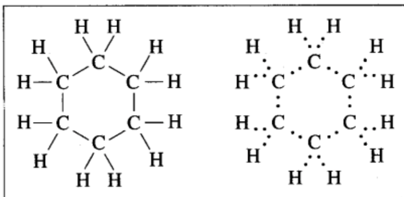
Cyclohexane
