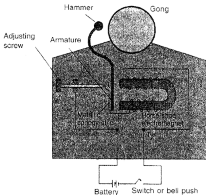
An electric bell
