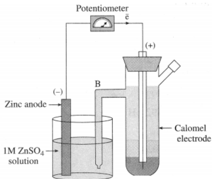
Fig. 5.15 : Determination of standard electrode potential using calomel electrode
