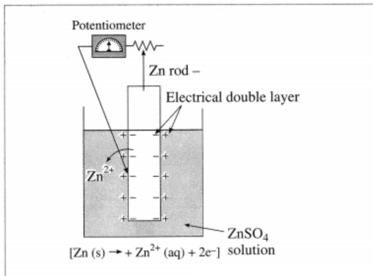
Fig 5.12(a) : Measurement of single electrode potential
