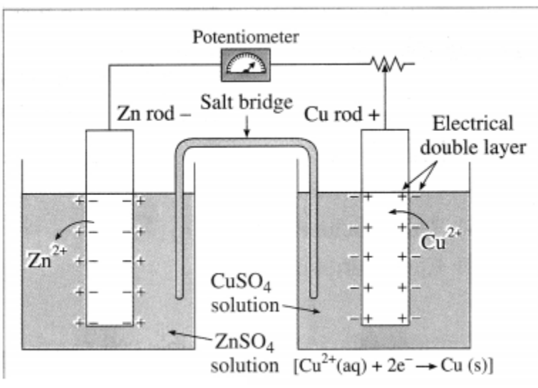
Fig 5.12(b) : Measurement of cell potential
