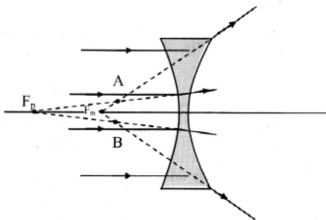
Spherical aberration in concave lens
