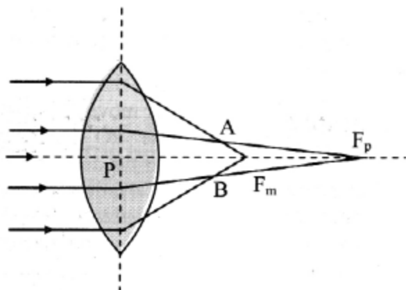
Spherical aberration in convex lens
